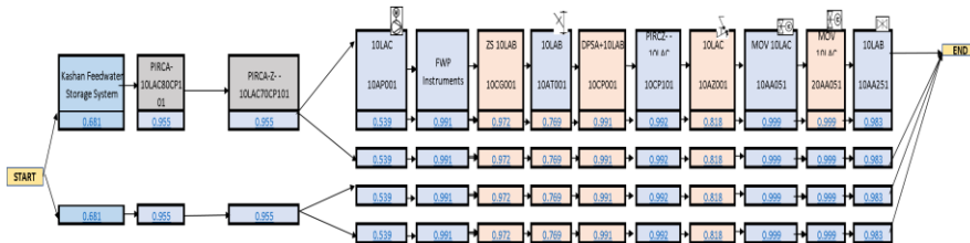
Fig2: Configuration of HRSG boiler water supply system in 4 pump mode
